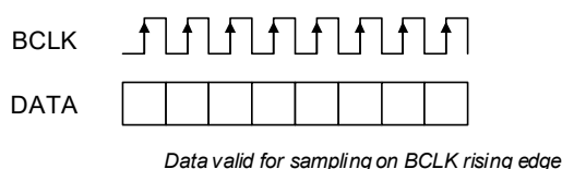
Figure 4-18. Noninverted BCLK
