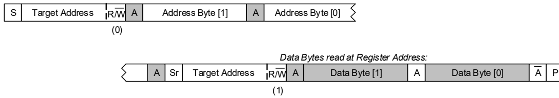
Figure 4-31. Single-Register Read from Specified Address
