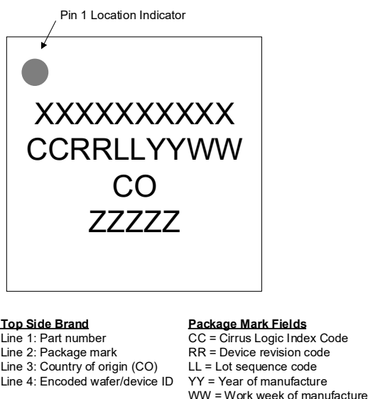
Figure 10-1. Package Marking
