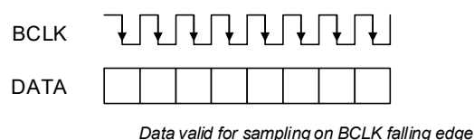
Figure 4-19. Inverted BCLK
